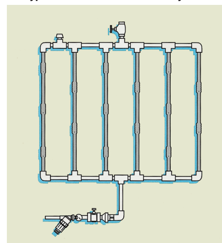
Typical outline of a subsurface system
